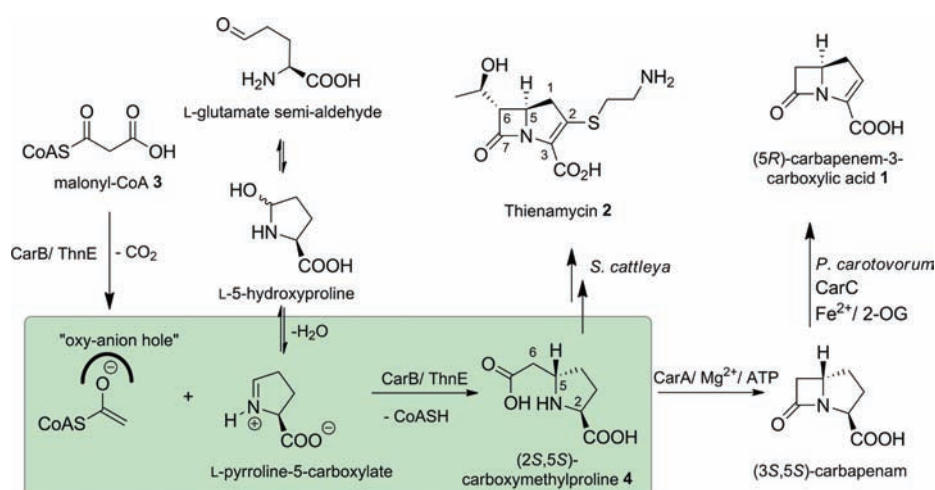
Scheme 1. Role of the Carboxymethylproline Synthases CarB and ThnE in the Biosynthesis of (5 R )-Carbapenem-2-em-3-carboxylic Acid 1 and Thienamycin 2, Respectively
