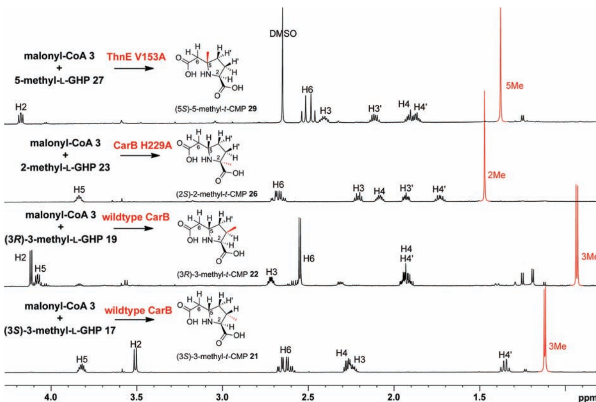
Figure 3. Spectroscopic analyses of the C2-, C3-, and C5-methyl-substituted- t -CMP products. 1 H NMR spectra of methylated- t -CMP derivatives resulting from incubation of malonyl-CoA 3 and the shown methylated-L-GHP derivatives in the presence of the shown CMPSs, under standard conditions.
